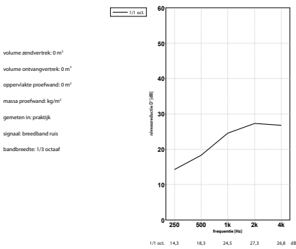
Silent series sound insulation capacity
